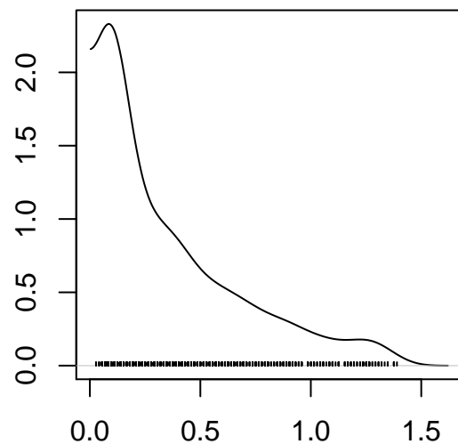
Density of Alpha1[factor1]
