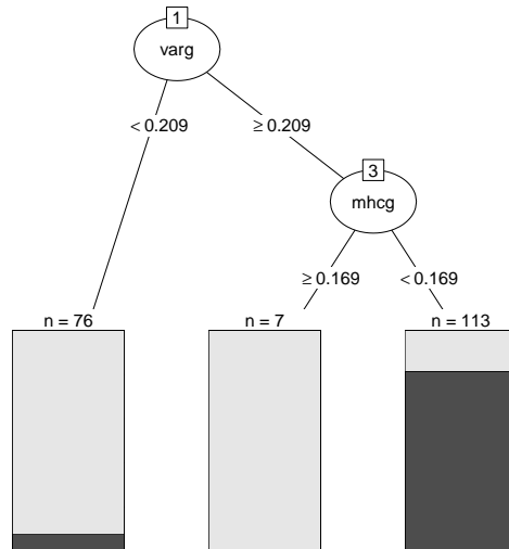
Figure 9.4 Pruned classification tree of the glaucoma data with class distribution in the leaves.
