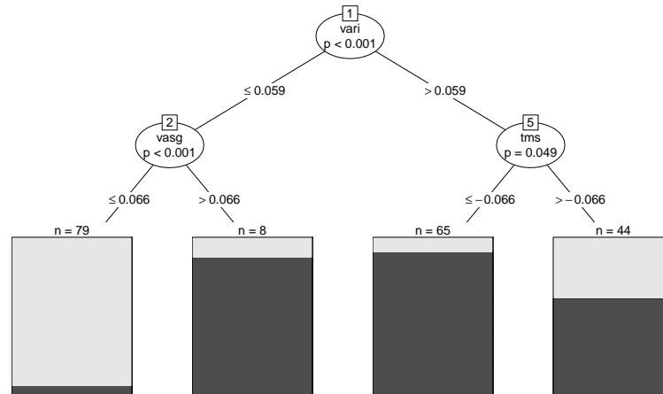
Figure 9.7 Conditional inference tree with the distribution of glaucomatous eyes shown for each terminal leaf.
