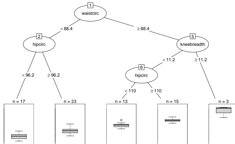
Figure 9.2 Pruned regression tree for body fat data.
