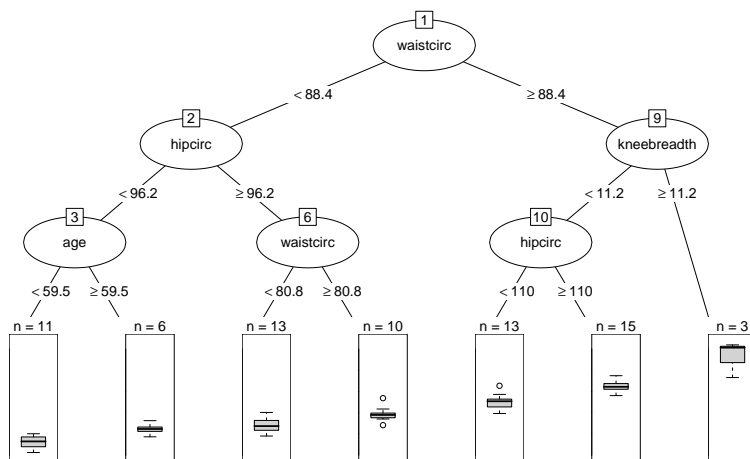
Figure 9.1 Initial tree for the body fat data with the distribution of body fat in terminal nodes visualized via boxplots.
