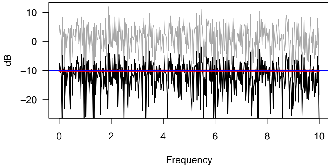
Figure 4: Rescaled PSD estimates for a single realization of a \mathcal{N}(0,1) process with a sampling rate of 20 \text{ s}^{-1} rather than 1 \text{ s}^{-1} as from before. The original spectrum (grey) is scaled to the appropriate level (black). The thick red line shows the mean (rescaled) spectral level, and the blue line shows the predicted mean value based on twice the sampling frequency.
