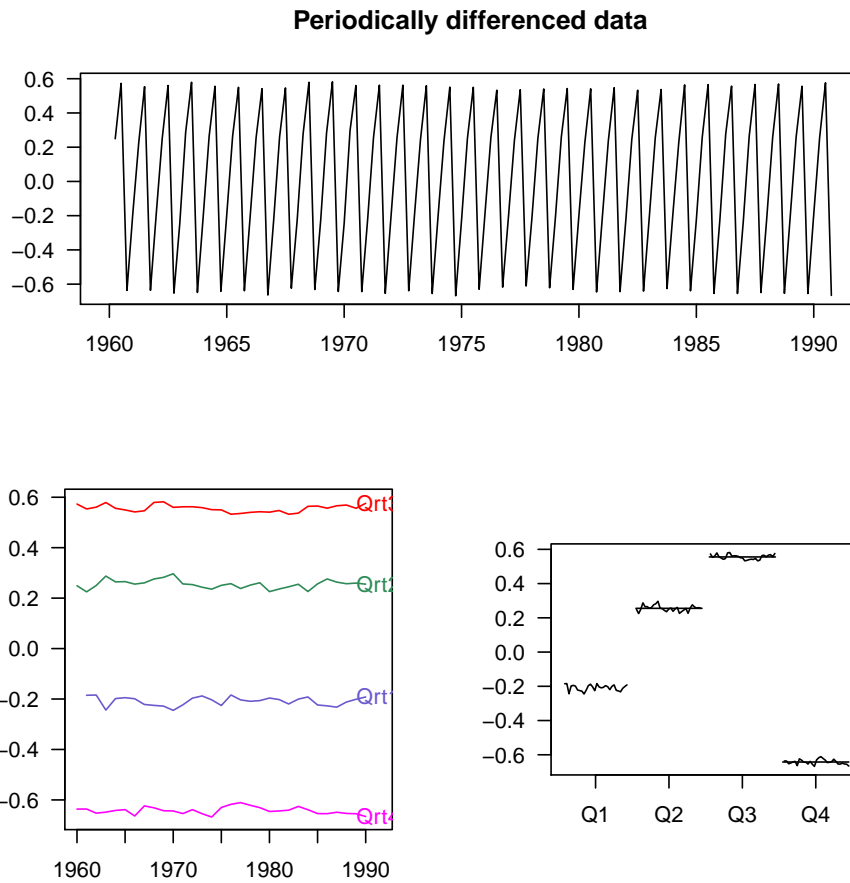
Figure 1: Periodically differenced data and seasonal paths
