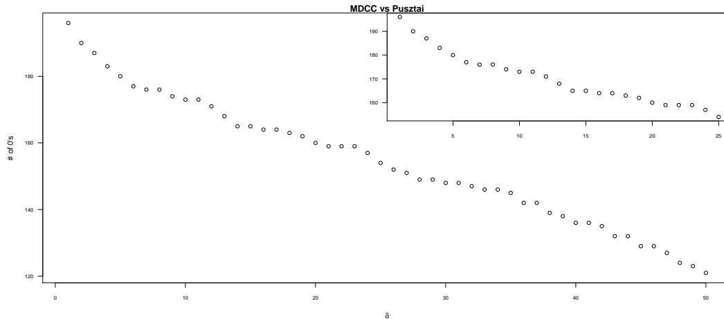
Figure 9: Deltaplot for lists MDCC vs. Pustztai for first 200 objects
