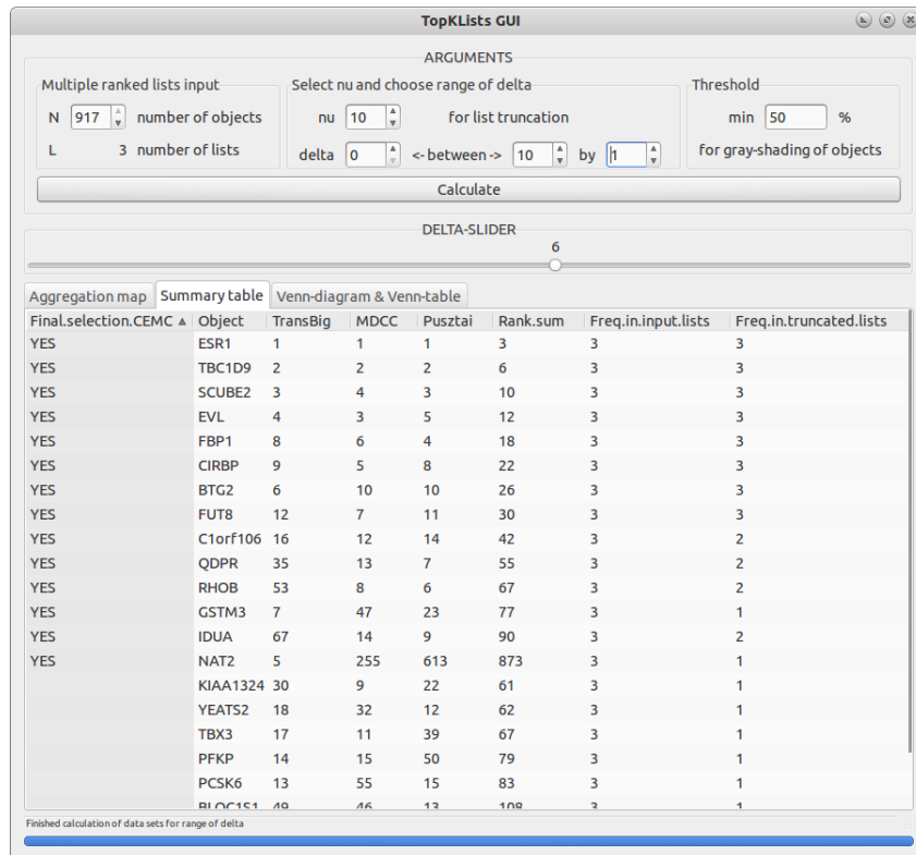
Figure 14: Summary table result of the TopKListsGUI
