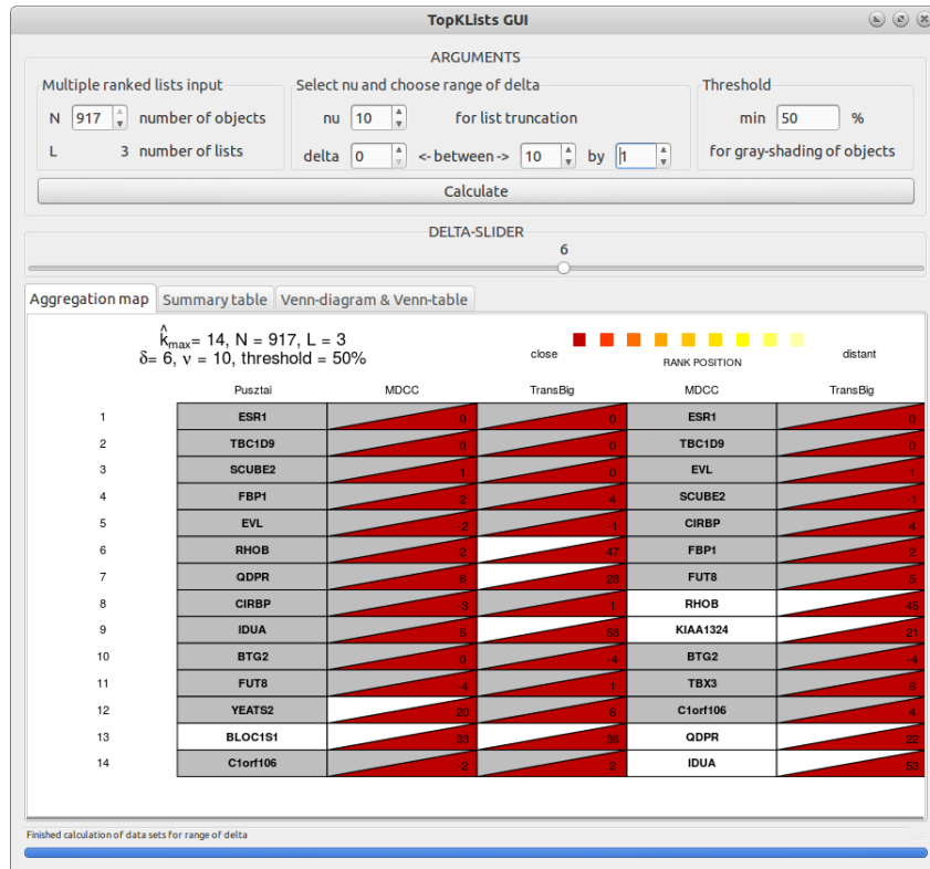
Figure 13: Aggregation map result of the TopKListsGUI
