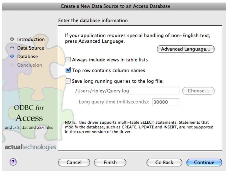
Figure 3: (Top) The main ODBC Administrator dialog box from a Mac OS X 10.5 system. (Bottom) A page of the dialog box to specify a DSN for the Actual Technologies Access/Excel driver.
