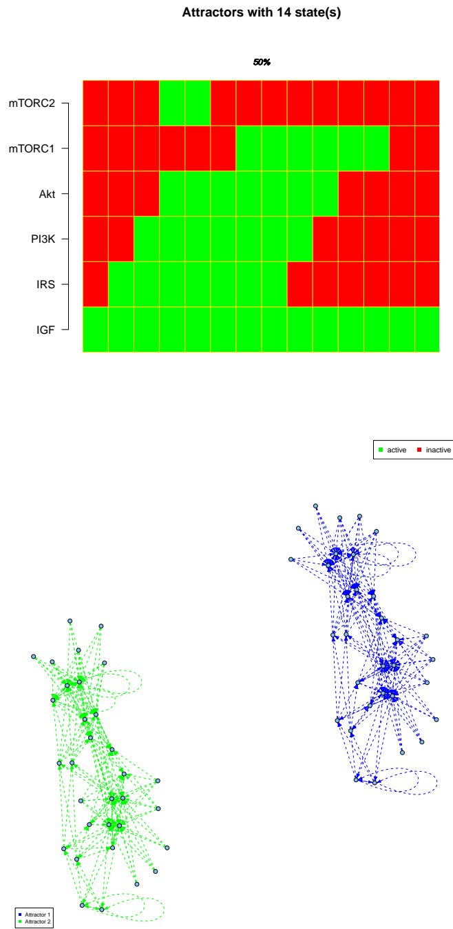
Figure 7: Top: Visualization of an attractor that describes the activation and inactivation of the PI3K-Akt-mTOR signalling cascade through IGF and IRS. The columns of the table represent consecutive states of the attractor. On top, the percentage of states leading to the attractor is supplied.
